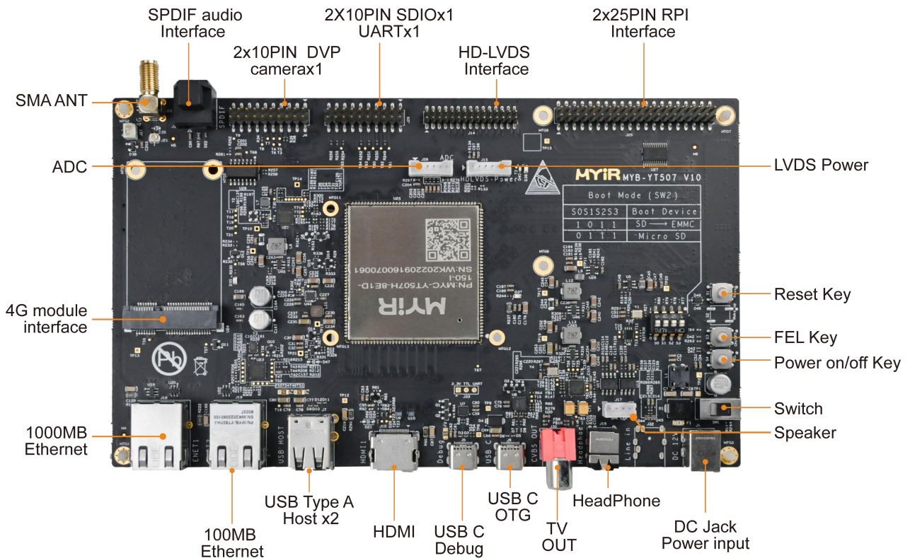
MYD-YT507H Development Board Top-view
