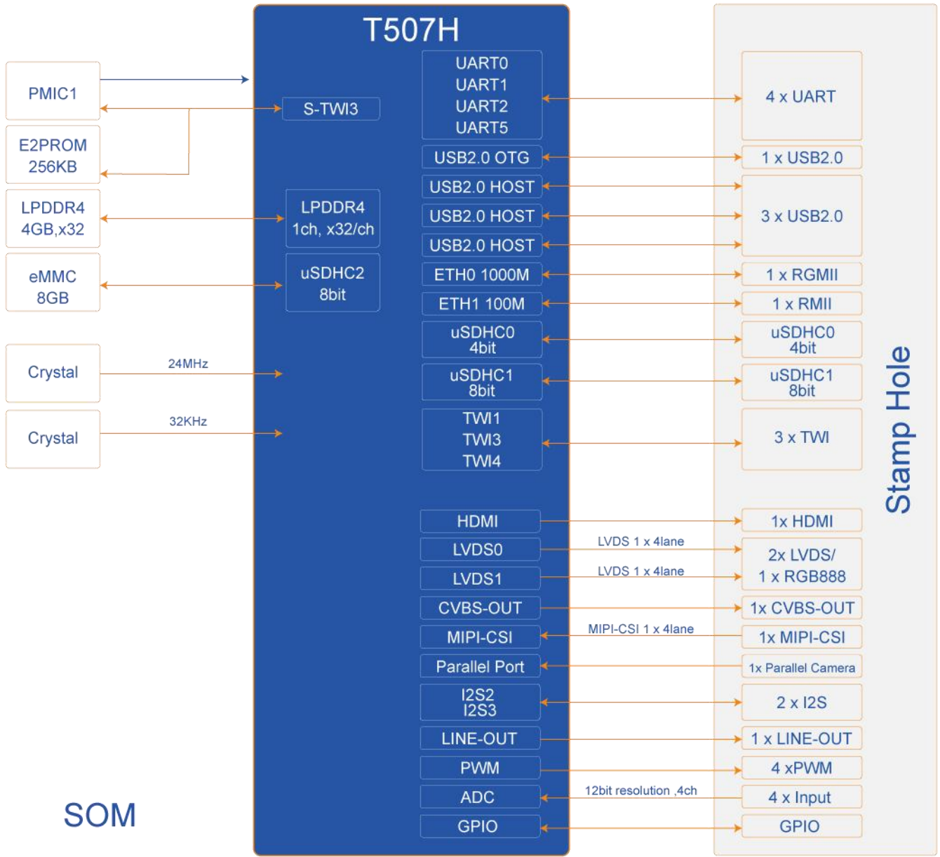
MYC-YT507H CPU Module Function Block Diagram
