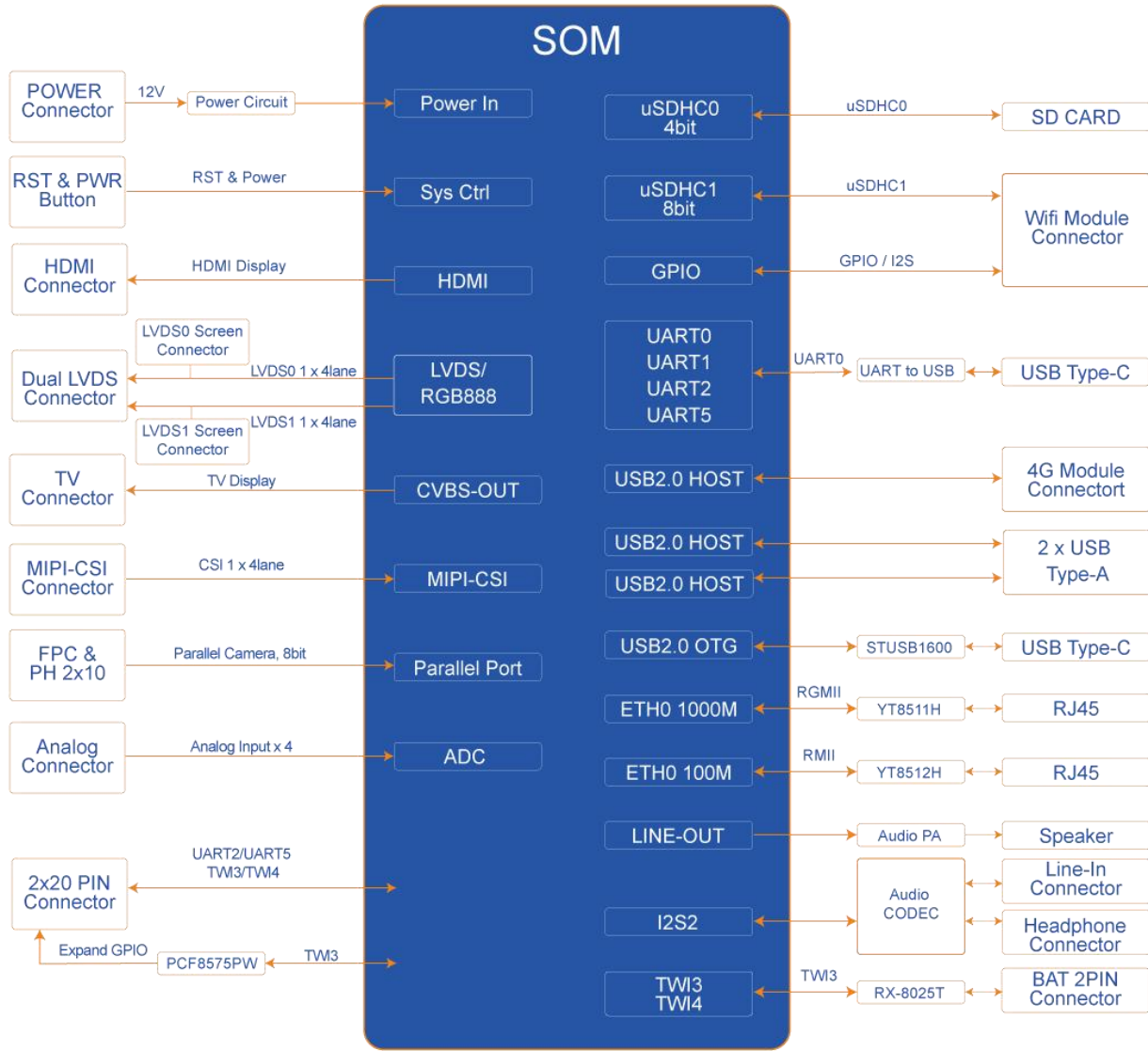
MYD-YT507H Development Board Function Block Diagram
