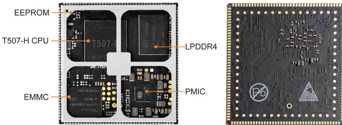
MYC-YT507H CPU Module Top-view and Bottom-view (delivered with shielding cover installed by default)
