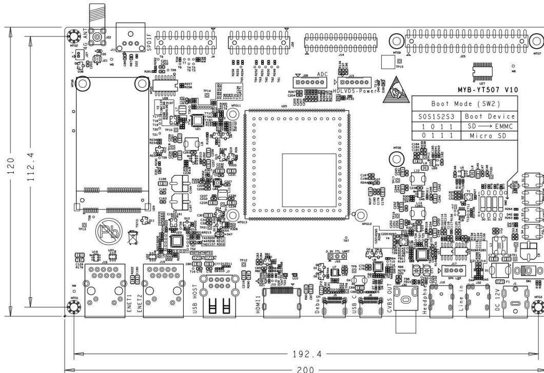
MYD-YT507H Base Board Dimensions Chart (Unit: MM)
