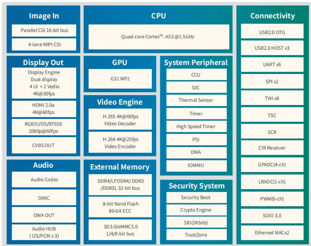
ALLWINNER T507-H Processor Block Diagram
