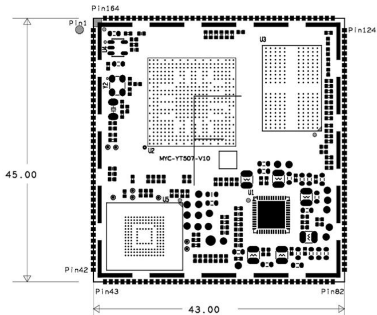
MYC-YT507H Dimensions Chart (Unit: MM)
